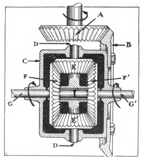
Fig. 7.—Bevel differential gears set.
